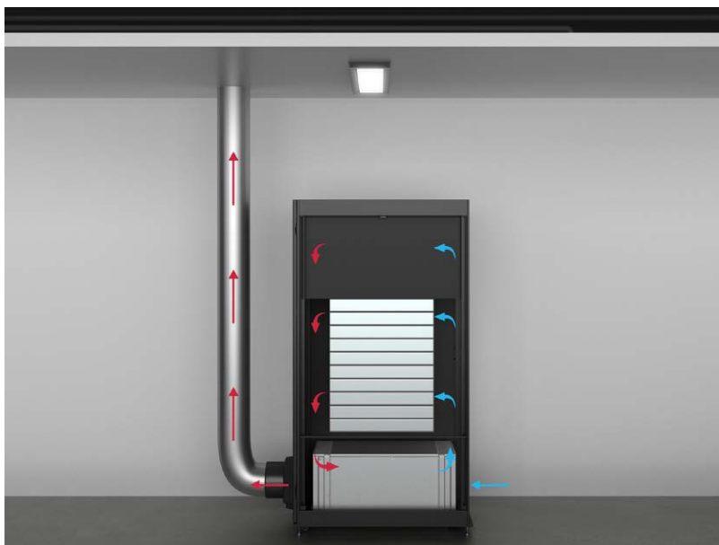
Heat rejected to ceiling plenum
