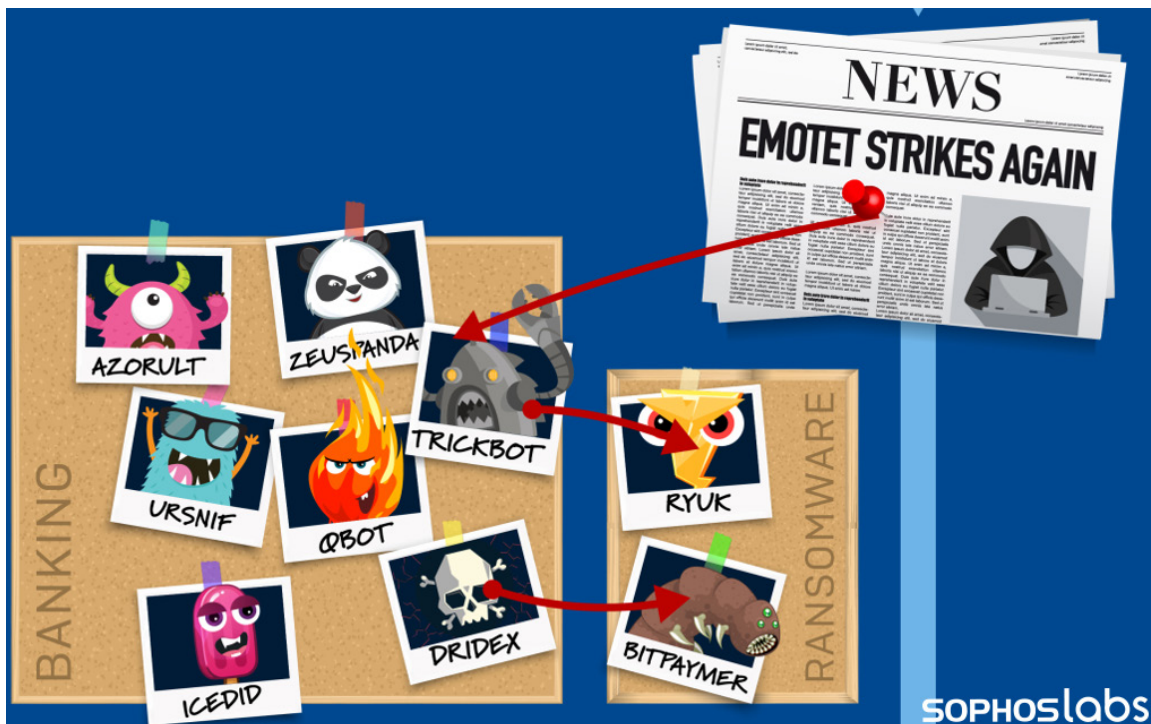
Fig.14. Source: SophosLabs.
