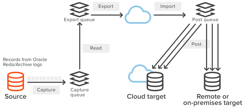
The SharePlex data replication process
