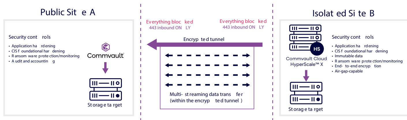
Figure 1 - Data isolation using direct connections
